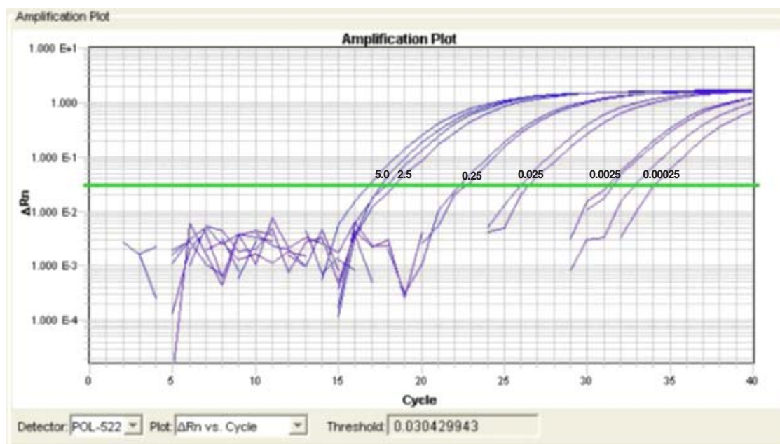
Figure 2. qPCR amplification curves for pollock genomic DNA standards ranging from 0.00025 – 5.0 ng \mu\text{l}^{-1} .
