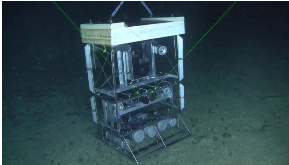
Figure 8. A surveillance platform resting on the seafloor. Lower level contains the computers and batteries, middle level contains the stereo cameras and other instrumentation, and upper level houses the DIDSON sonars and the strobe for the cameras. Image was taken from the manned submersible. For reference, the green lasers are 20 cm apart.
