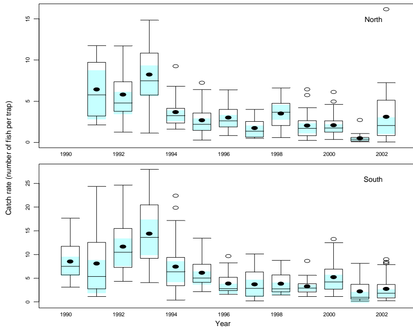
Figure 2: Distribution of sablefish survey catch rates (number of fish per trap) for each set by year and stock. Boxplots show the distribution of catch rates observed on each set. The filled circles show the mean annual catch rate. The lightly shaded rectangle indicates an approximate 95% confidence interval on the median annual catch rate.
