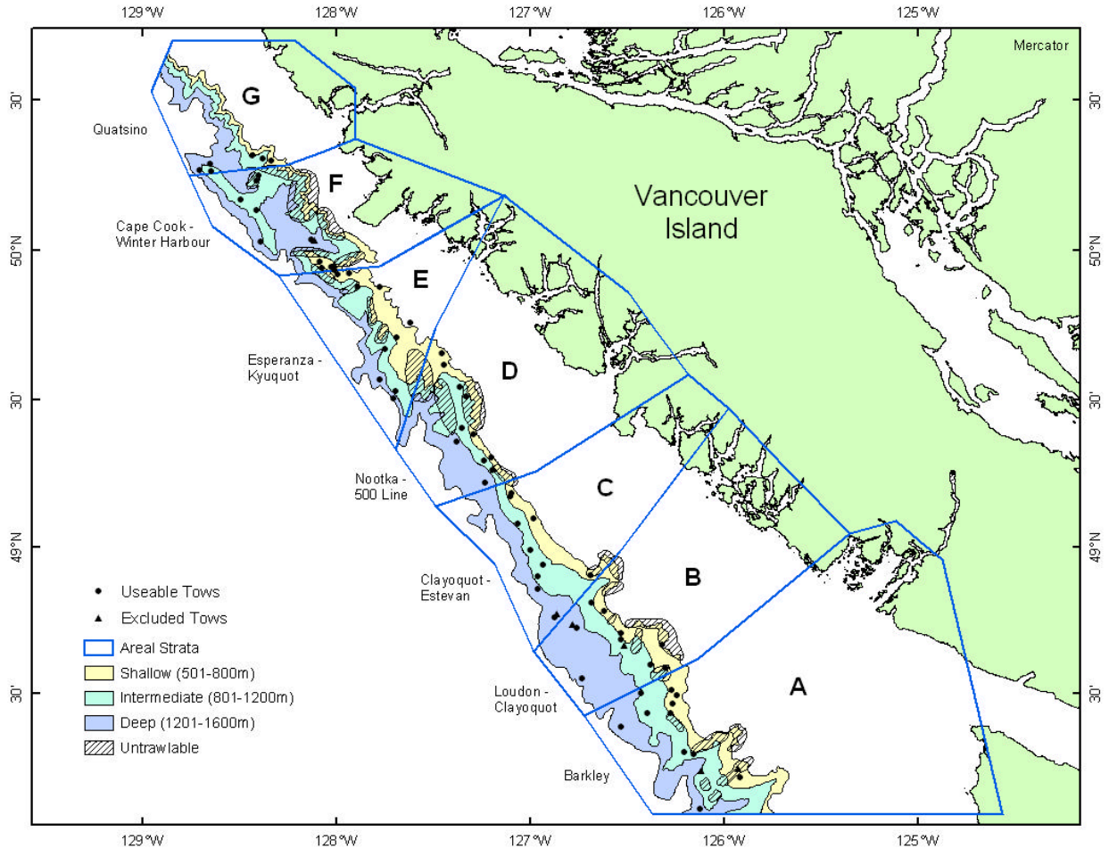
Figure 1. Longspine thornyhead survey (2002) with 7 areal strata (A-G) and 3 depth strata (501-800 m, 801-1200 m, 1201-1600 m). Number of tows = 74 (7 discarded).
