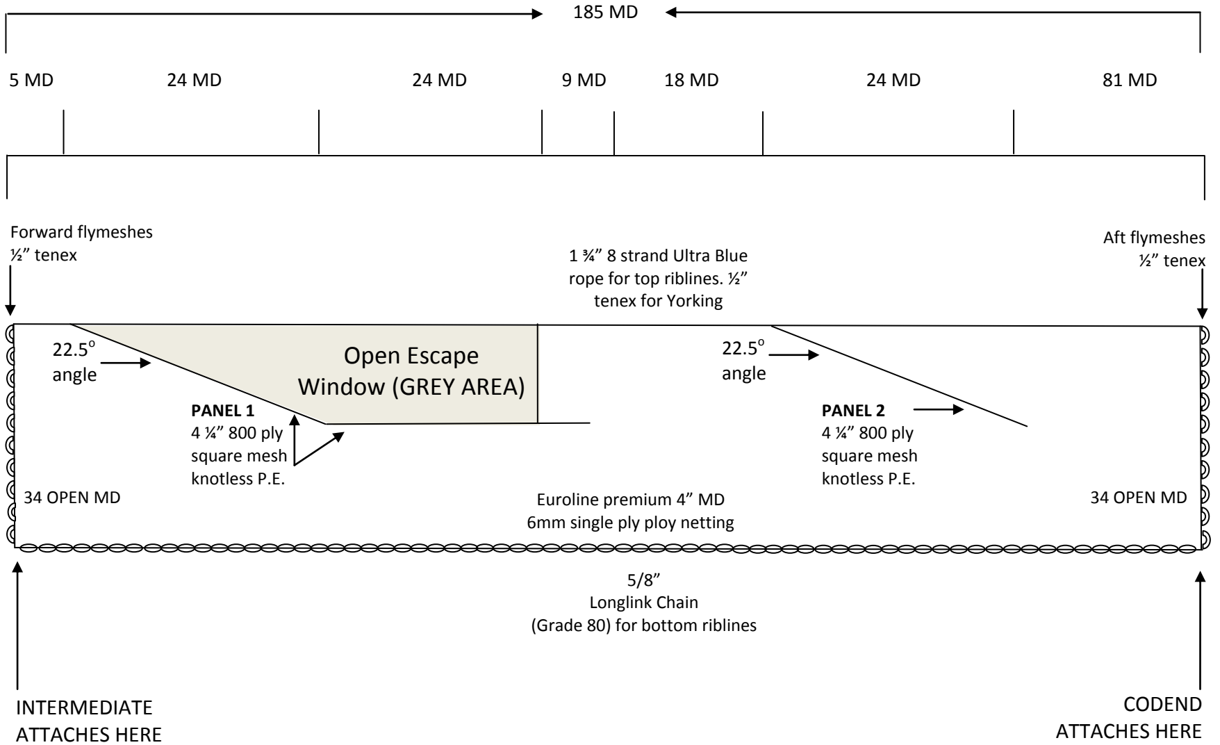
Figure 1. Bycatch reduction device diagram.
